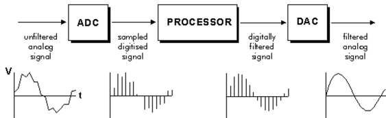
Conversion of signals
