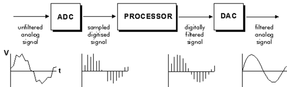
Conversion of signals
